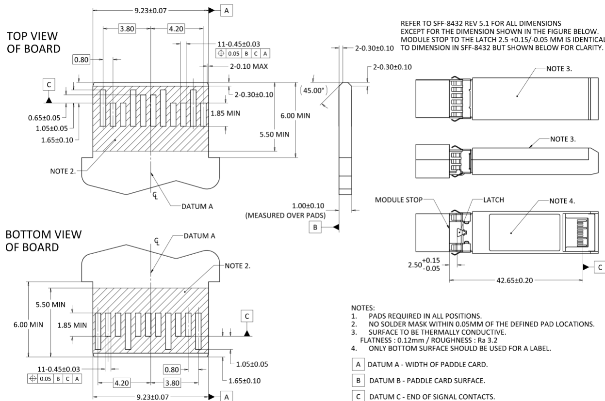
Figure 20: DSFP Module Card Edge and Mechanical
