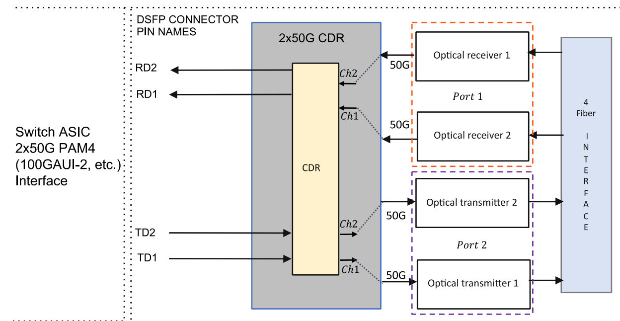
Figure 2: Block diagram for 100GBASE-SR2
