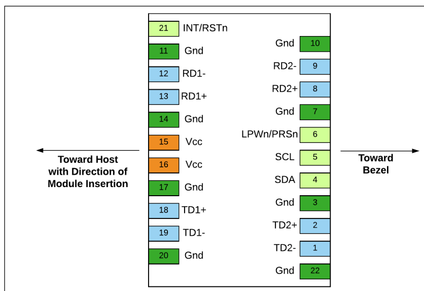
Figure 7: DSFP Host PCB pad assignment top view
