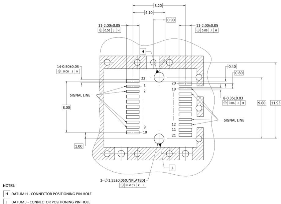
Figure 22: DSFP SMT Connector PCB Layout
