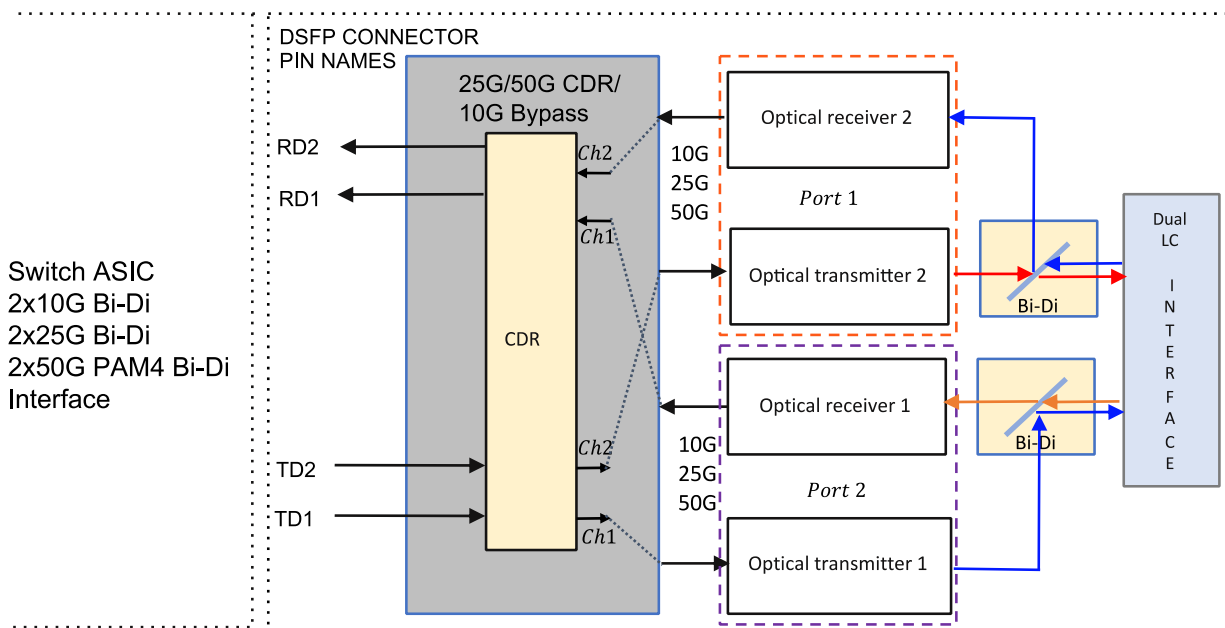
Figure 5: Block diagram for 10G/25G-NRZ and 50G-PAM4 Bi-Di
