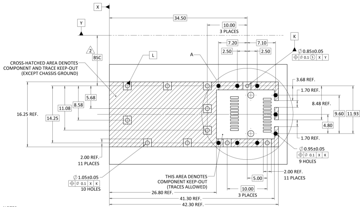
Figure 22: DSFP SMT Connector PCB Layout
