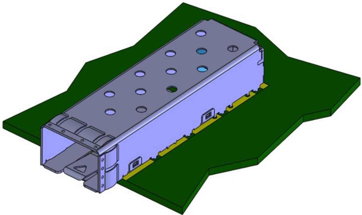
Figure 17: DSFP Press fit Cage
