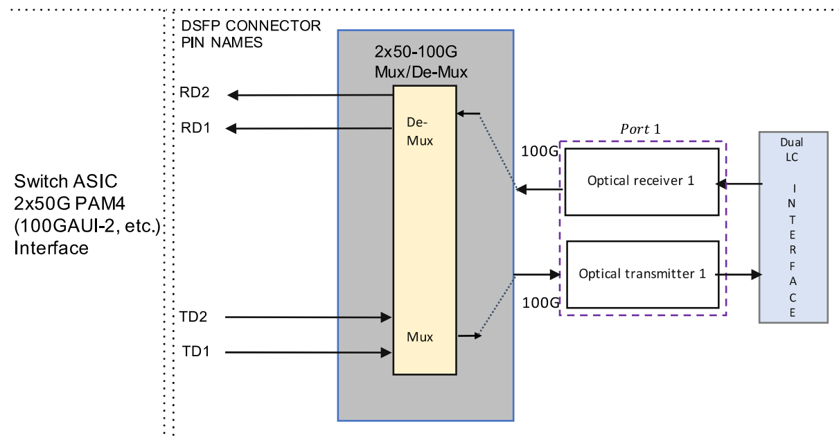
Figure 4: Block diagram for 100GBASE-DR
