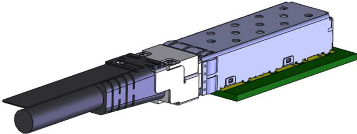
Figure 16: DSFP Module and Cage
