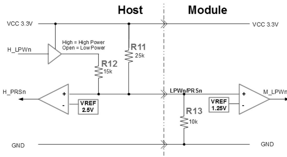
Figure 10: LPWn/PRSn circuit
