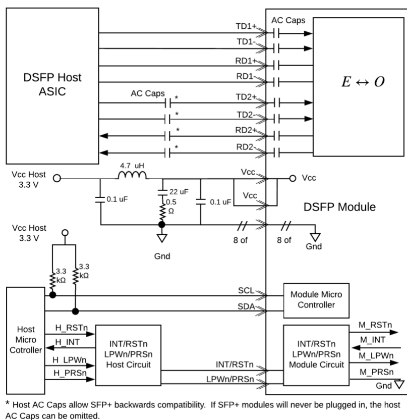
Figure 14: DSFP Host Application Reference with DSFP Module
