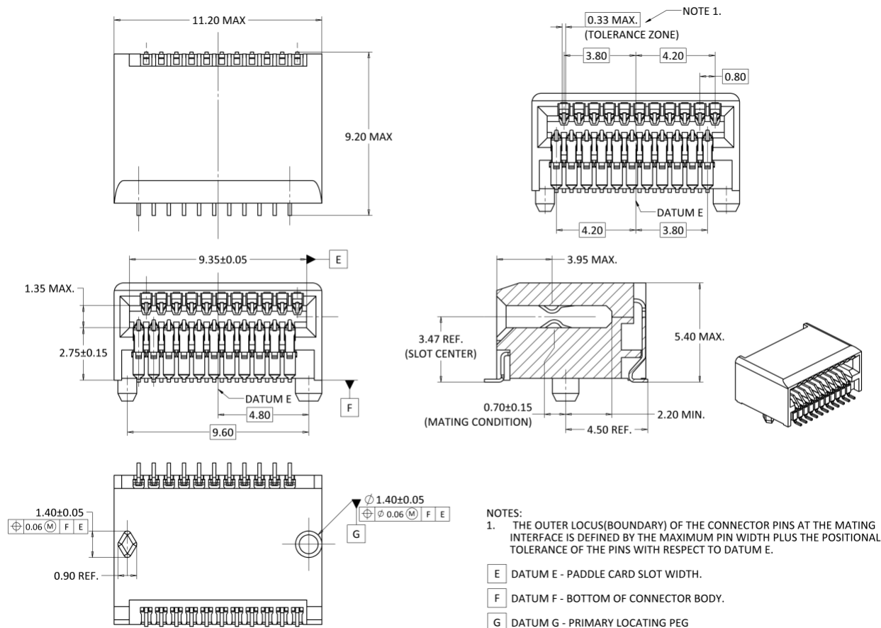
Figure 21: DSFP SMT Connector
