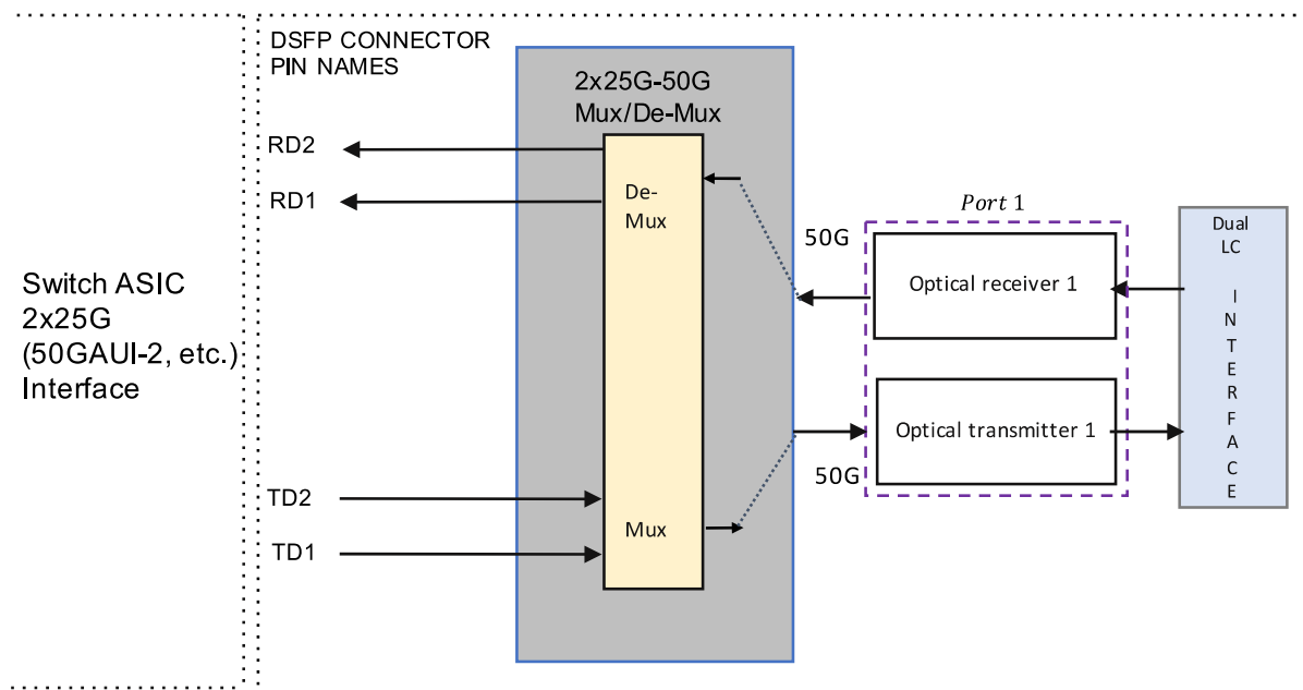
Figure 3: Block diagram for 50GBASE-SR/FR/LR with 2:1 mux
