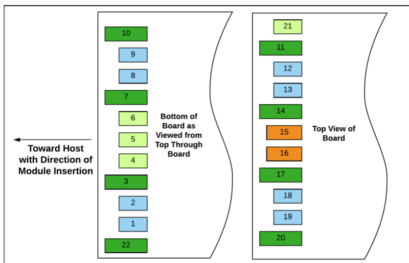
Figure 8: DSFP module contact assignment
