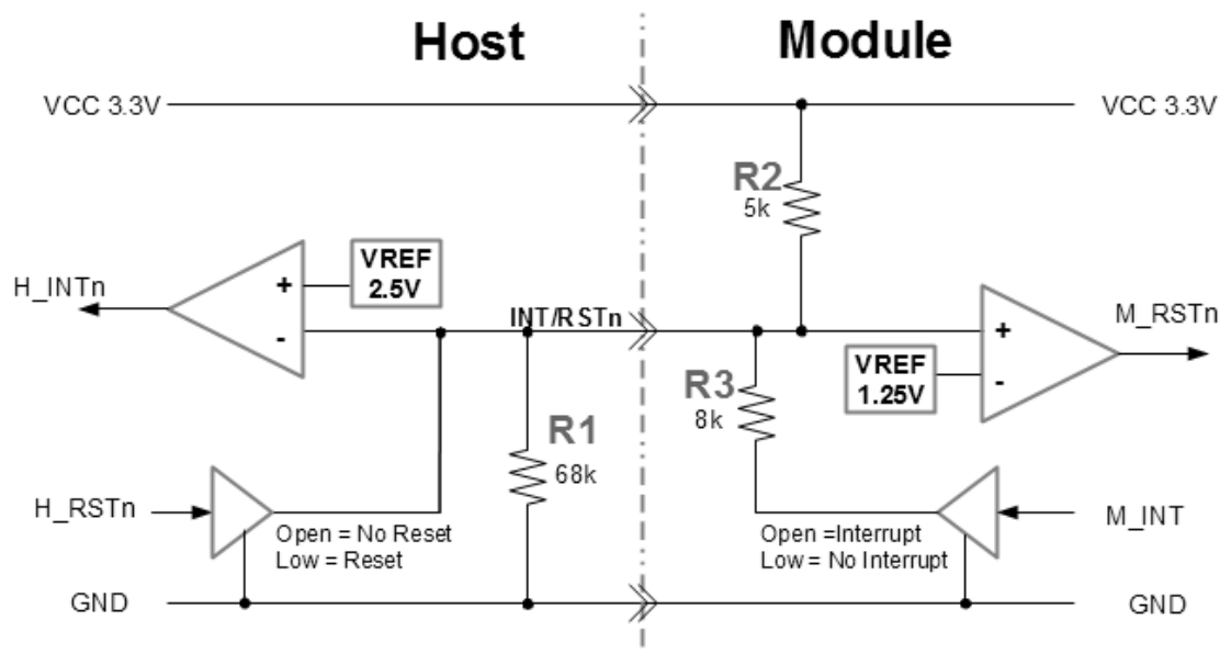
Figure 12: INT/RSTn circuit
