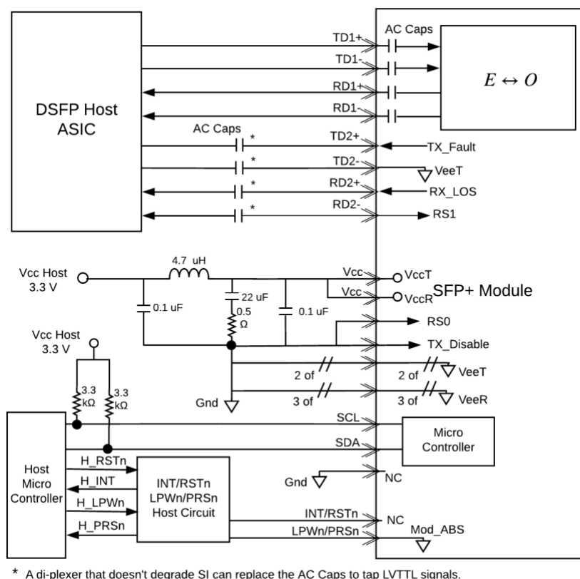
Figure 15: DSFP Host Application Reference with SFP+ Module
