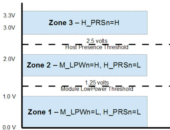
Figure 9: LPWn/PRSn voltage zones
